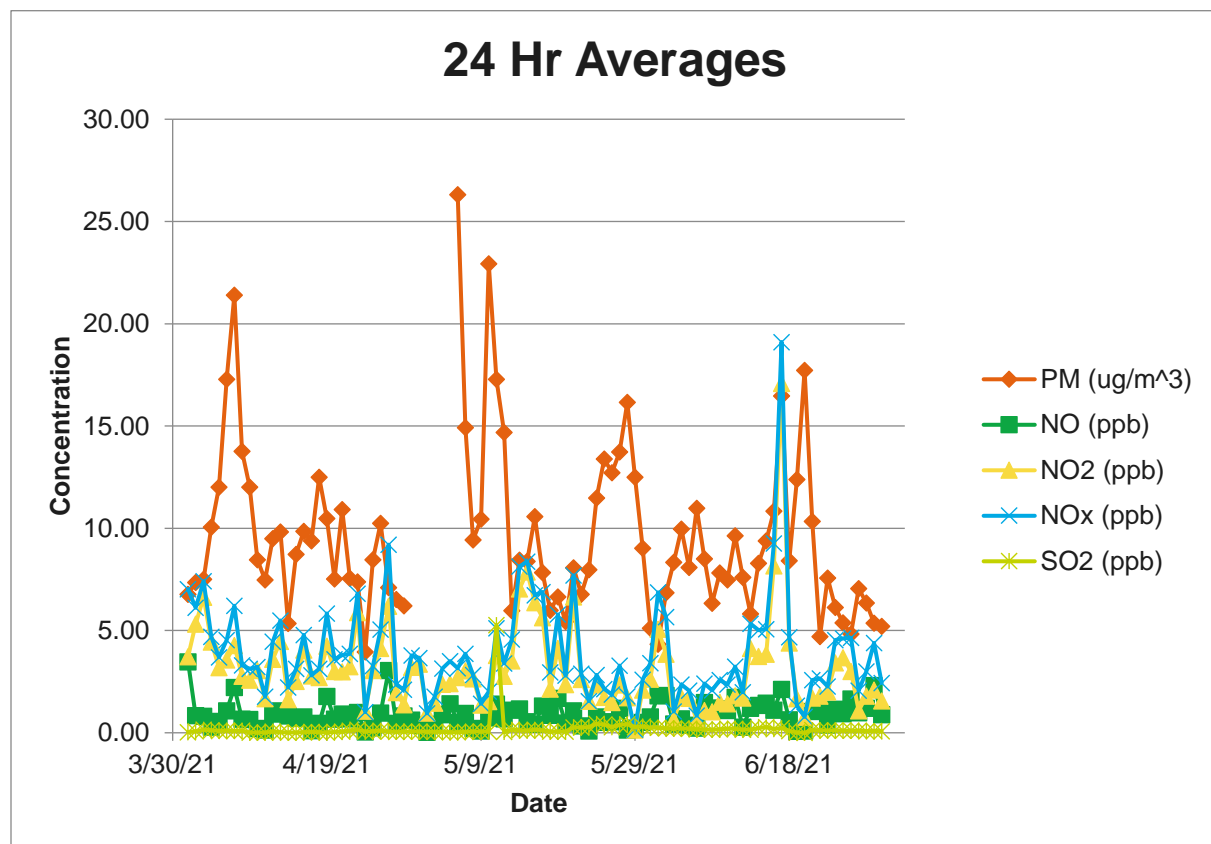
Figure 2-1. 24-hour Averages
