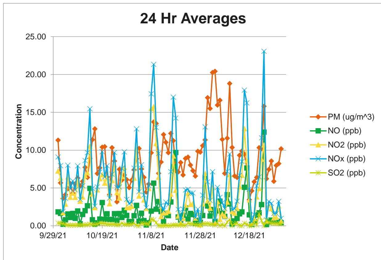
Figure 2-1. 24-hour Averages
